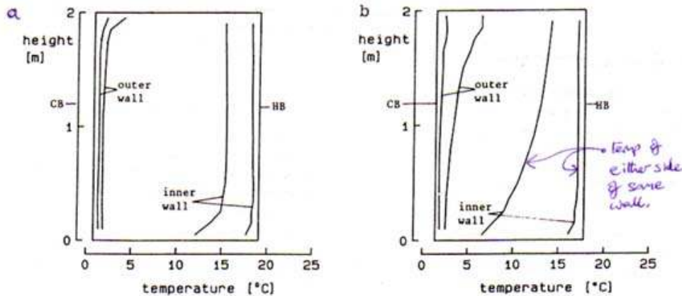
Fig. 2. Measured temperature profiles, gaps at top and bottom: (a) gaps=0 mm; (b) gaps=10 mm
