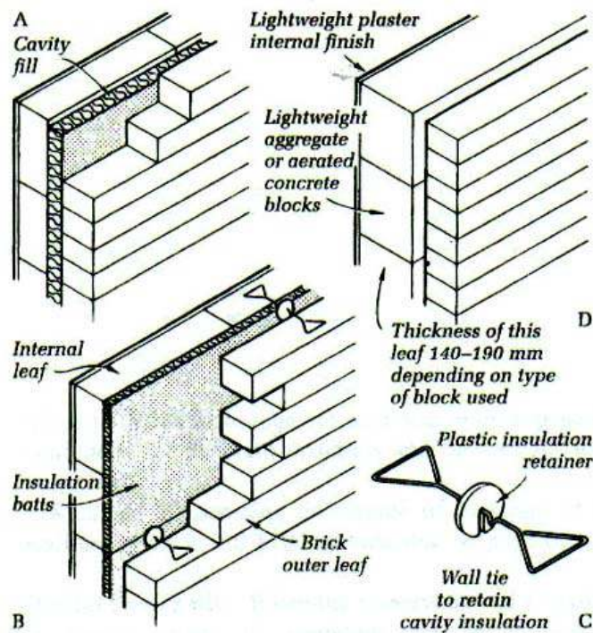
Figure 5.12 Thermal insulation of cavity walls
